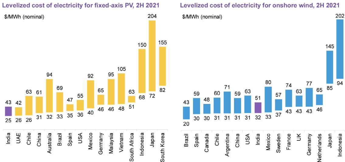
Fig. 9. India's solar and wind costs
